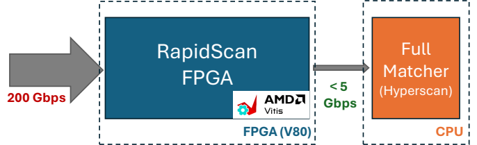
Fig. 1: RAPIDSCAN String Matching operates at over 200Gbps using less than 30% of the Versal V80. Along with Hyperscan on the host CPU, the system, RAPIDDETECT, can process incoming logs at over 160Gbps on a single server
