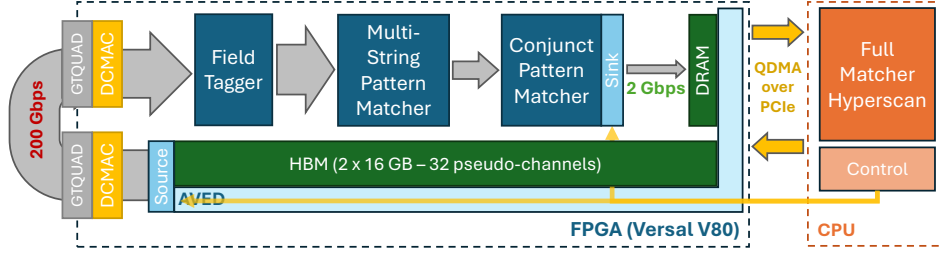
Fig. 6: RAPIDDETECT System Prototype implemented on the Versal V80 with 200G Ethernet
